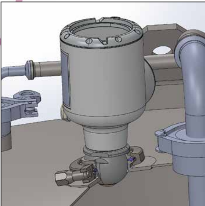
Krohne Radar Sensor with Multi-Flange
