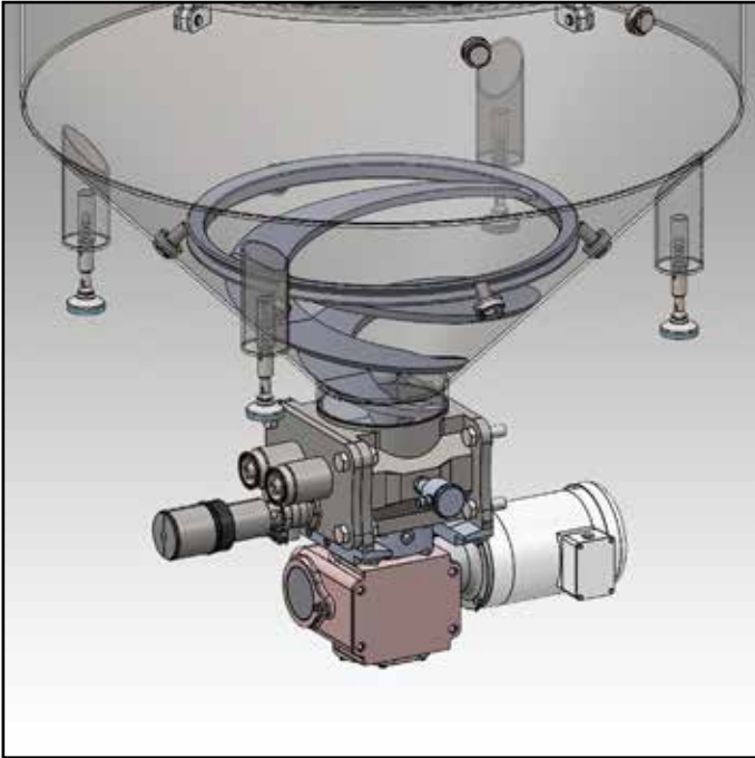
GS-Fusion used with Auger Housing
