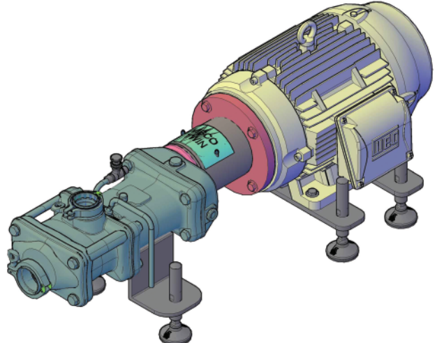
Frame #2 Frameless (w/Six Legs)
