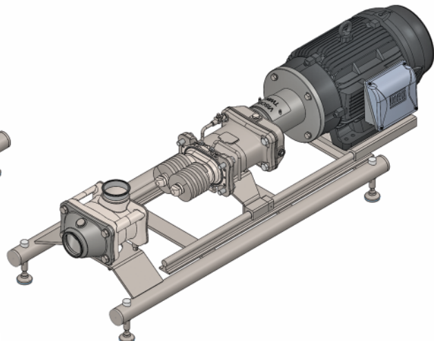
Frame #4 Slider Mount
