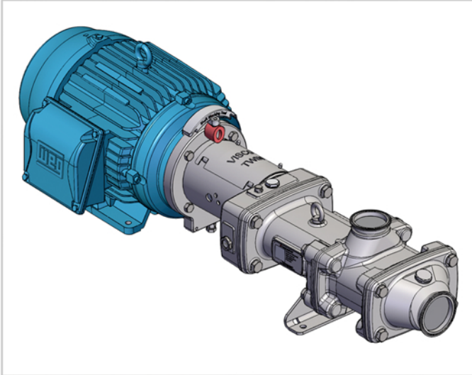
Frame 1 (Frame for Skid Mount)
